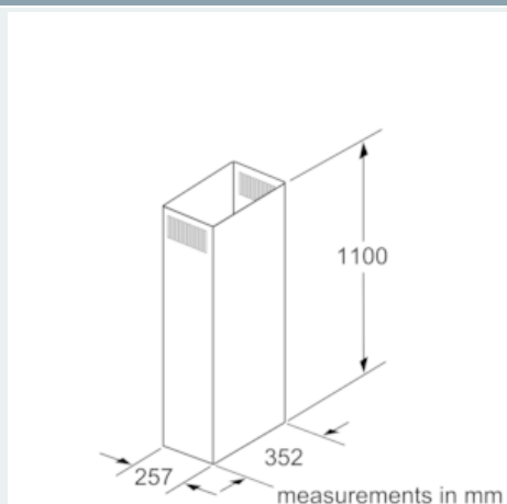
Dimensioned drawings
