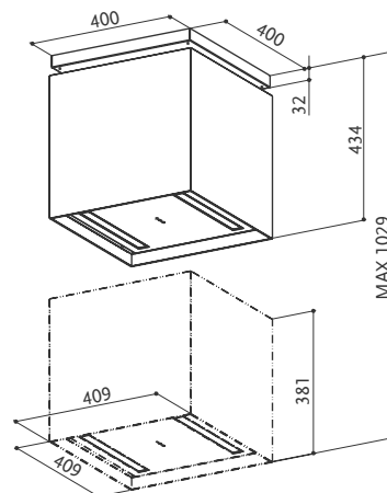
Lybra, ducted version
