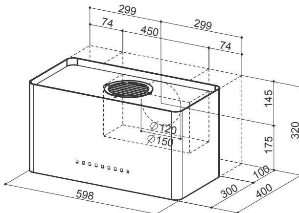
Air outlet adjustable on the rear side
